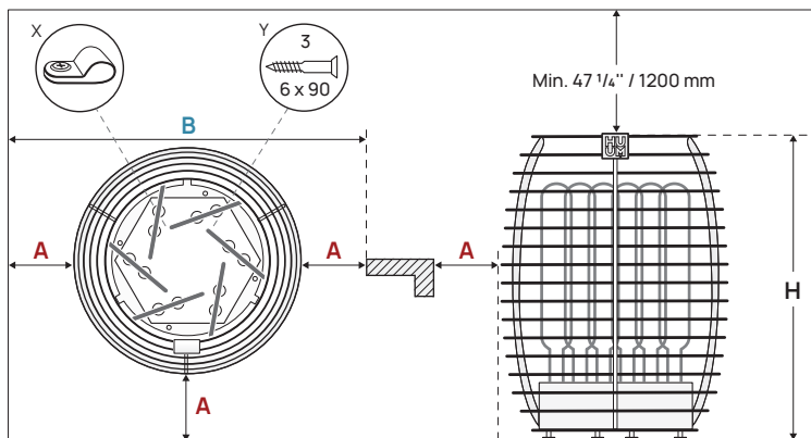
Figure 1 Positioning of the heater
